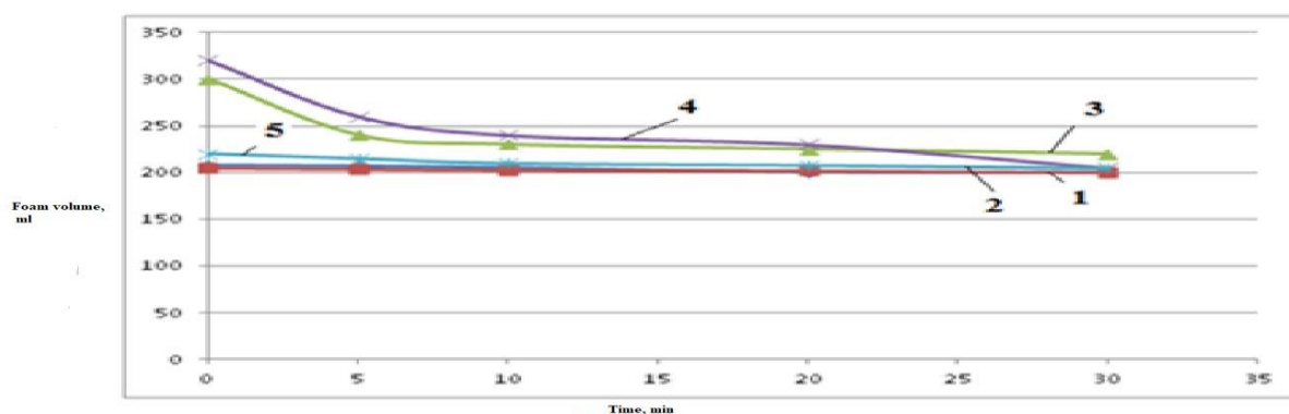
Fig. 2. Kinetics Of Foam Stability Of Solutions Of Flotation Reagents-Foaming Agents On A Water-Alcohol Basis
