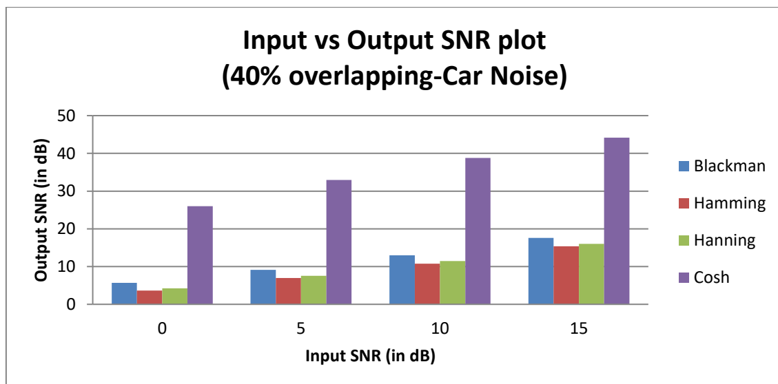
Fig.4. Input vs Output SNR plot
