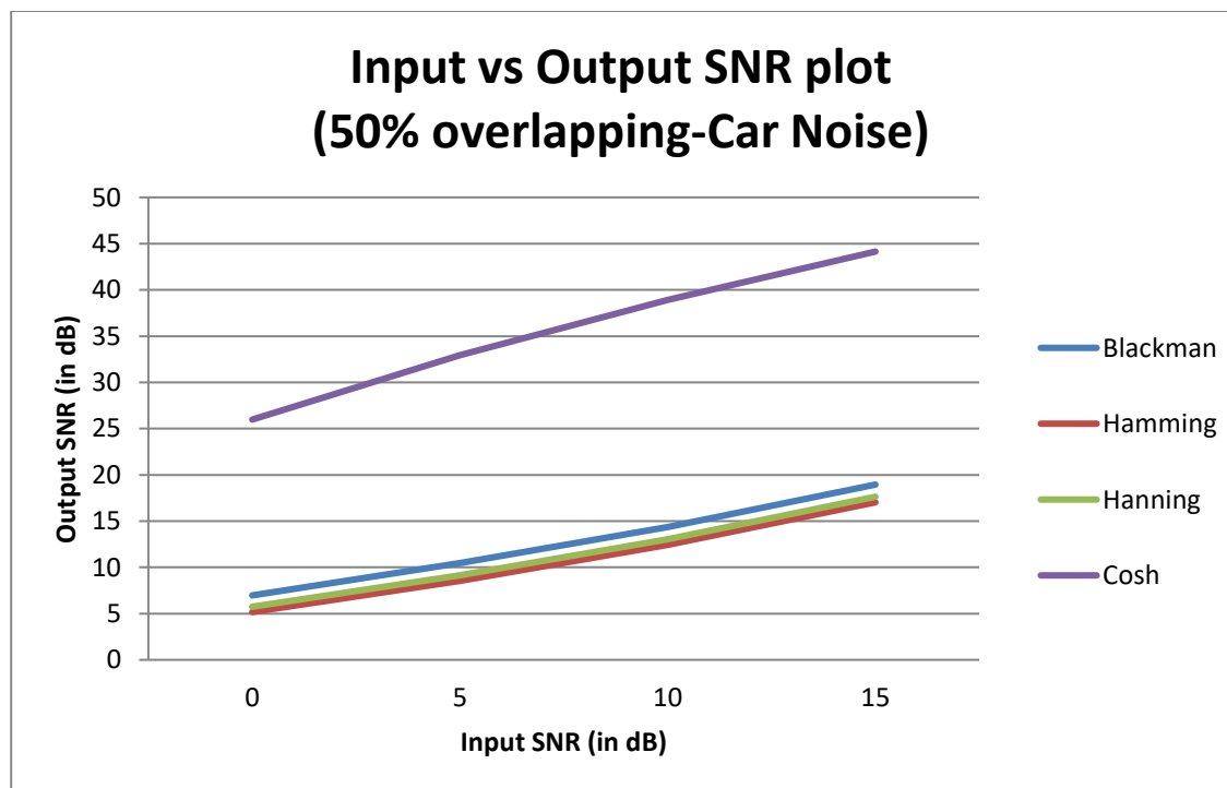
Fig.5. Input Vs. Output SNR plot
