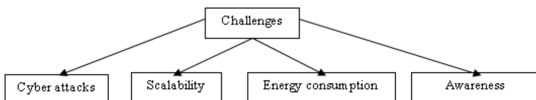
Fig 8: Blockchain challenges
