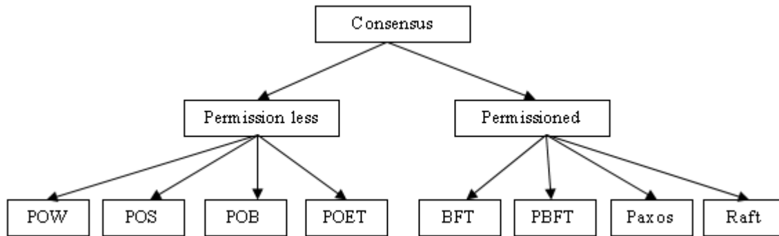
Fig 6: Blockchain consensuses
