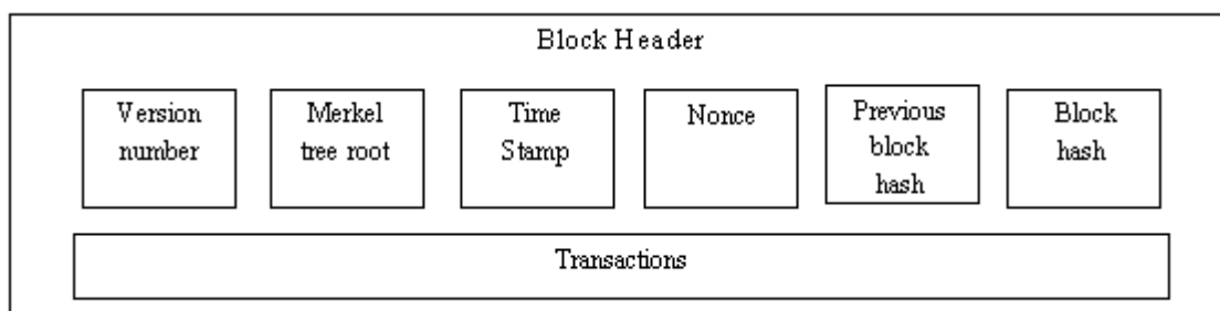
Fig 2: Block Structure
