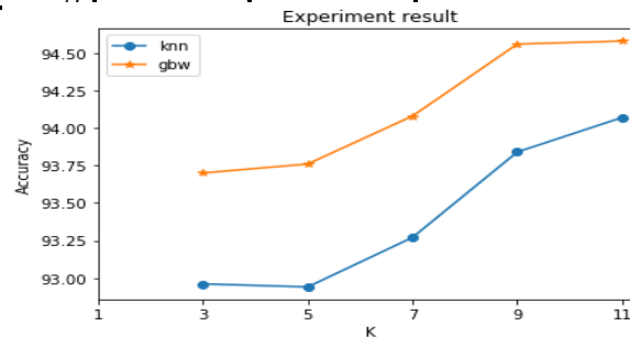
Figure2.Result of Breast Cancer Dataset
