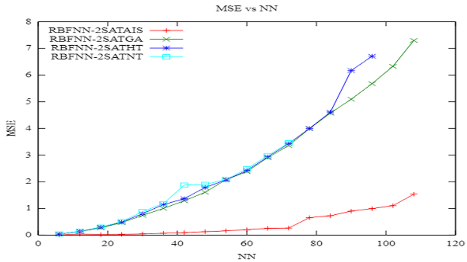
Figure 1. MSE value of the entire models of RBFNN-2SAT
