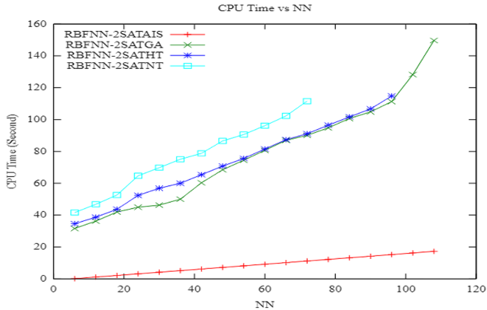
Figure 4. CPU time (seconds) models of RBFNN-2SAT
