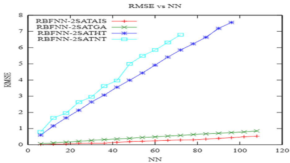
Figure 2. RMSE value of the entire models of RBFNN-2SAT
