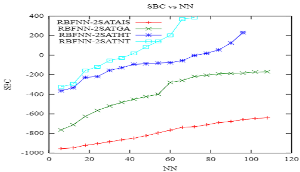
Figure 3. SBC value of the entire models of RBFNN-2SAT
