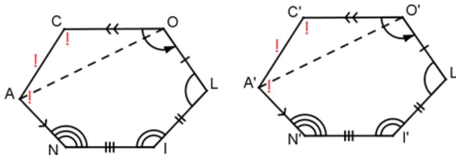
Figure 8. hex COLINA \cong hex C'O'L'I'N'A' by 5S-4A Convex Hexagon Congruence Theorem
