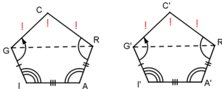
Figure 4. \text{pen } CRAIG \cong \text{pen } C'R'A'I'G' by 3S-4A Convex Pentagon Congruence Theorem
