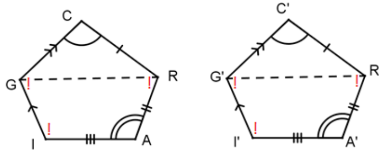
Figure 5. pen CRAIG \cong pen C'R'A'I'G' by 5S-2A Convex Pentagon Congruence Theorem
