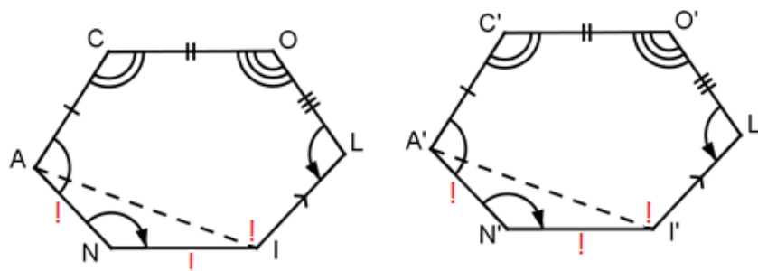
Figure 7. \text{hex } COLINA \cong \text{hex } C'O'L'I'N'A' by 4S-5A Convex Hexagon Congruence Theorem
