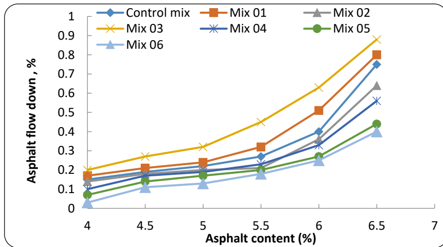
Figure 7 The drain down results
