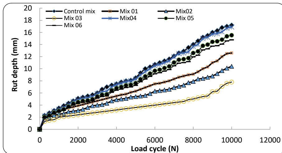
Figure 10 Rut depth values versus load cycle for various porous asphalt mixtures at 60 °C temperature
