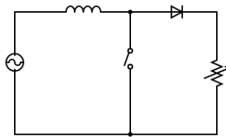
Fig.2. Basic Structure of Boost Converter
