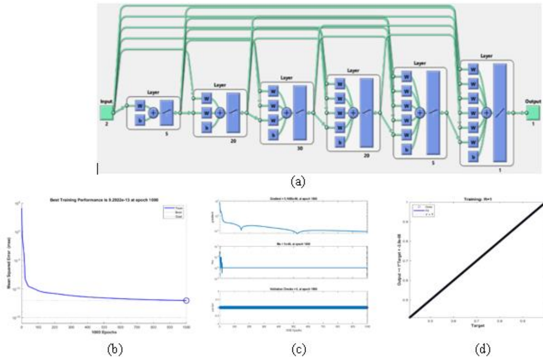
Fig.6. CFNN Control Design Parameters
