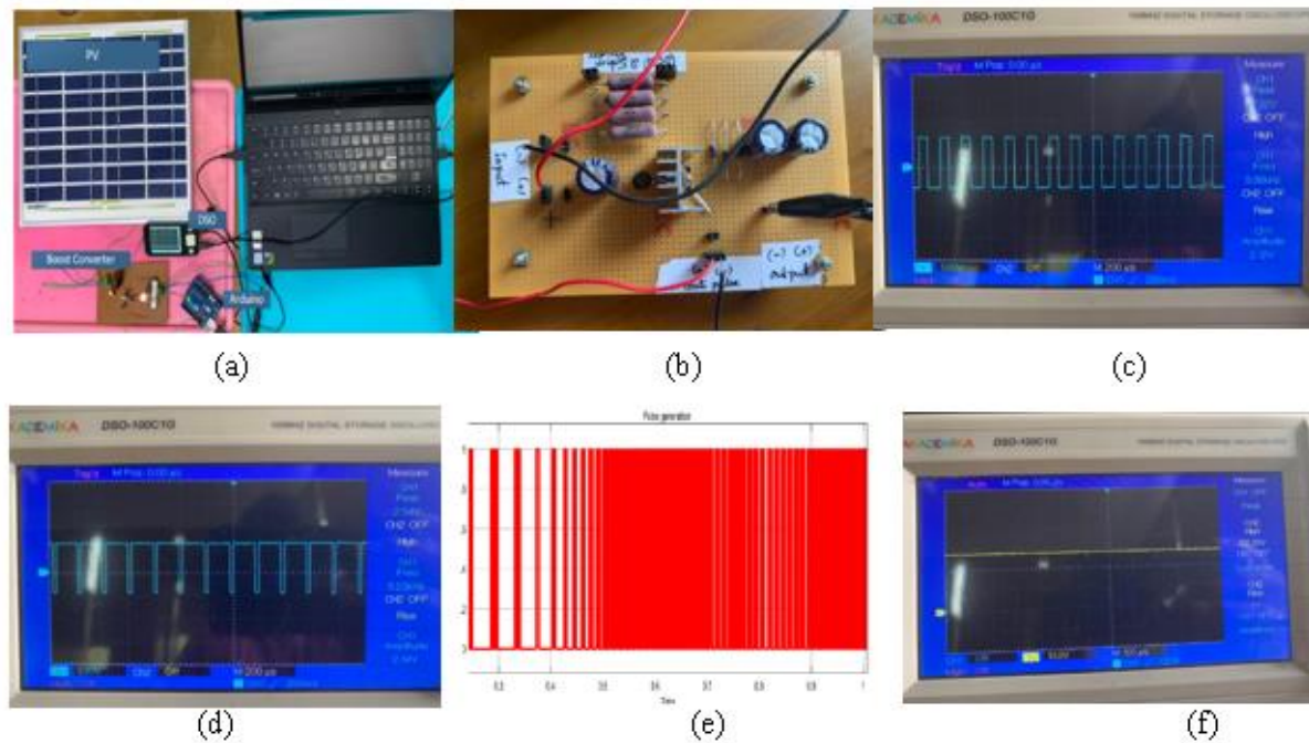
Fig. 12 Hardware Results
