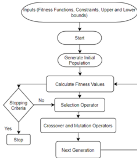
Fig.4. Flowchart for Genetic Algorithm
