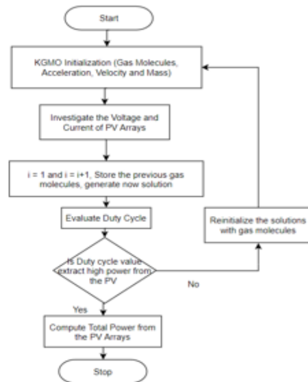
Fig.5. Flowchart for KGMO Algorithm
