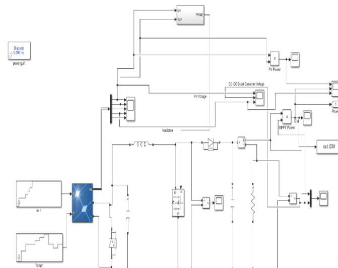
Fig.7. Simulation model 10 kW PV system for Various MPPT Algorithms
