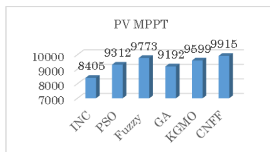
Fig 13. Comparative analysis of various MPPT techniques.
