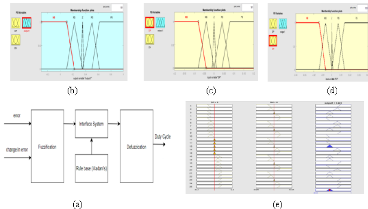
Fig.3. Fuzzy Logic Controller design parameters
