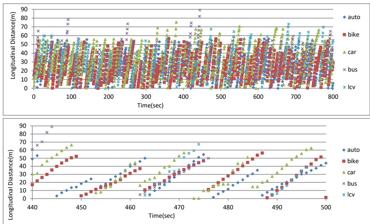
Fig.7: Time-Space diagram
