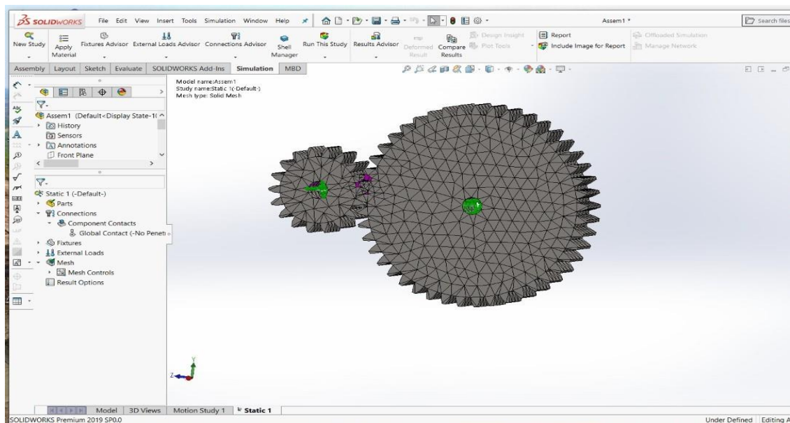
Figure 1. Meshing model
