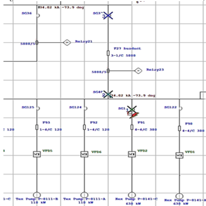
Figure 3: Simulation for Grid connected mode of operation when symmetric fault occurs.
