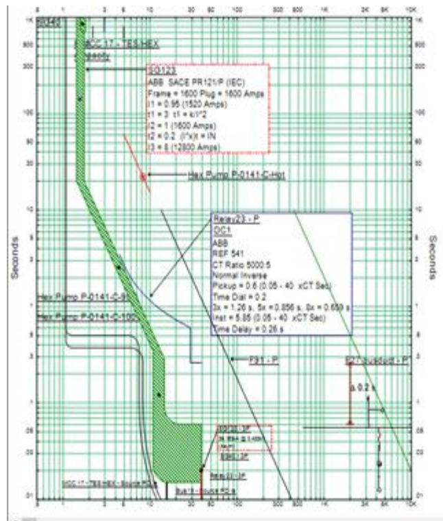
Figure 4: Sequence of operation and TCC star view Islanded mode of operation
