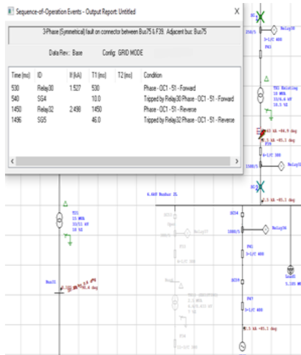
Figure 2: Simulation represents the symmetric fault occurs on conductor between Bus75 and Fd39.
