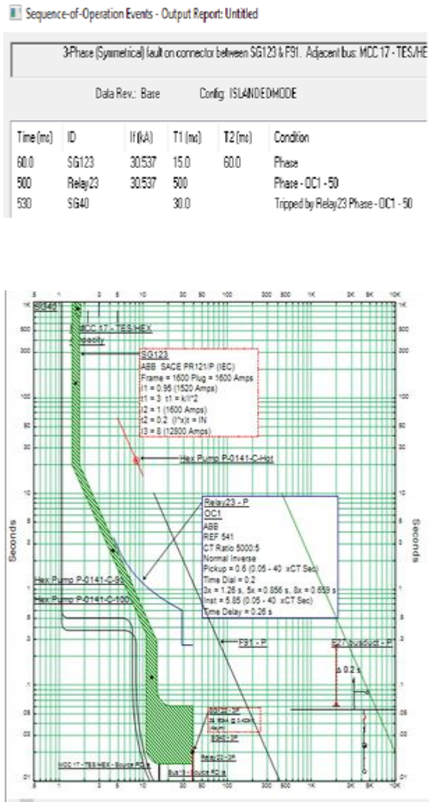
Figure 6: Sequence of operation and tcc star view
