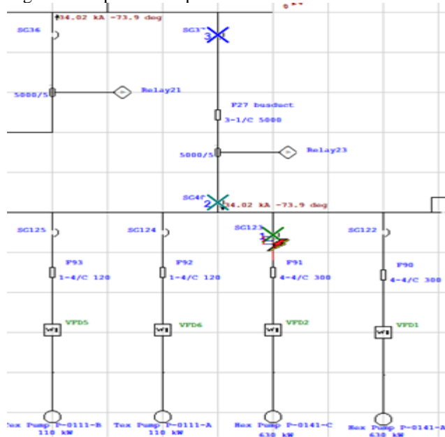
Figure 5: Simulation for islanded mode of operation when symmetric fault occurs.
