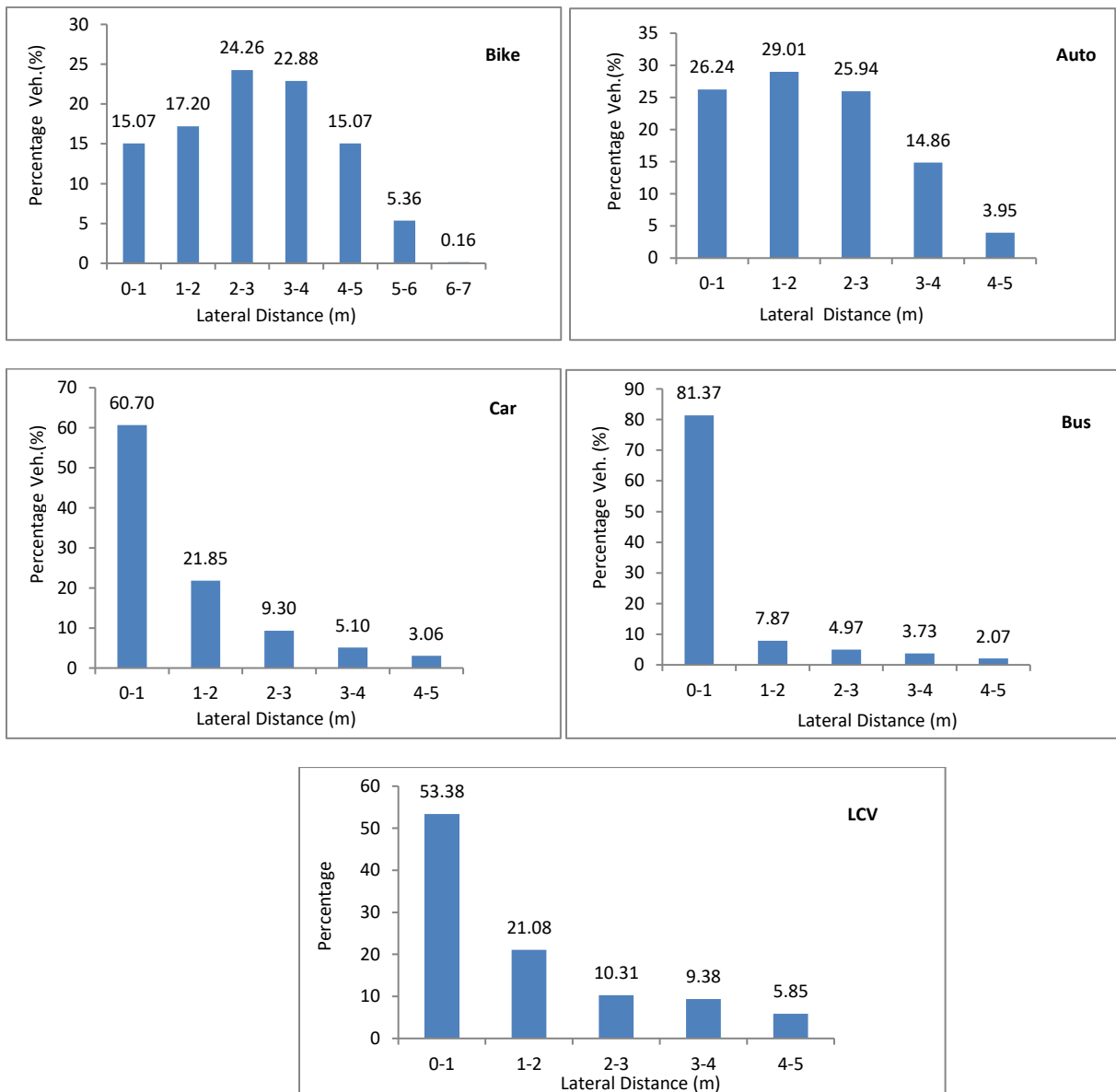
Fig.8: Lateral Displacements Of Vehicles From Median Side
