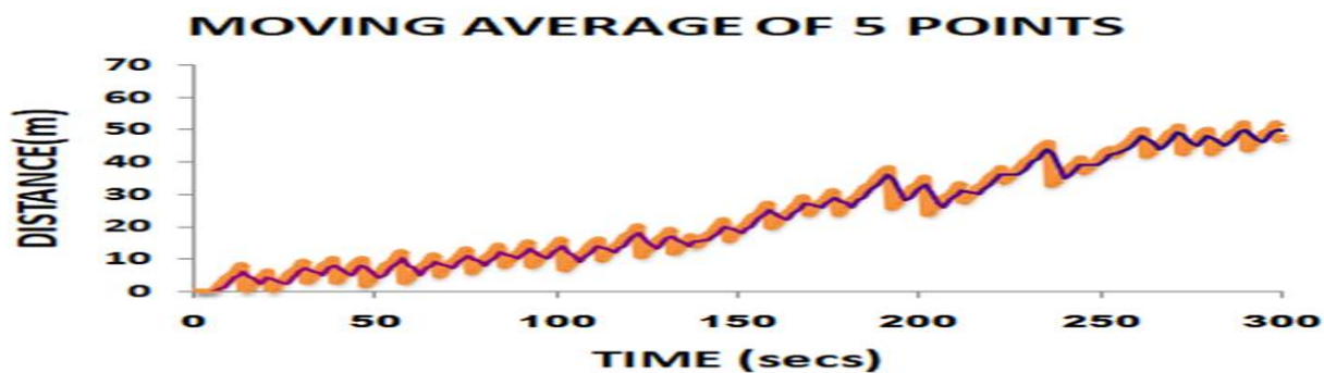
Fig. 6: Data Smoothing
