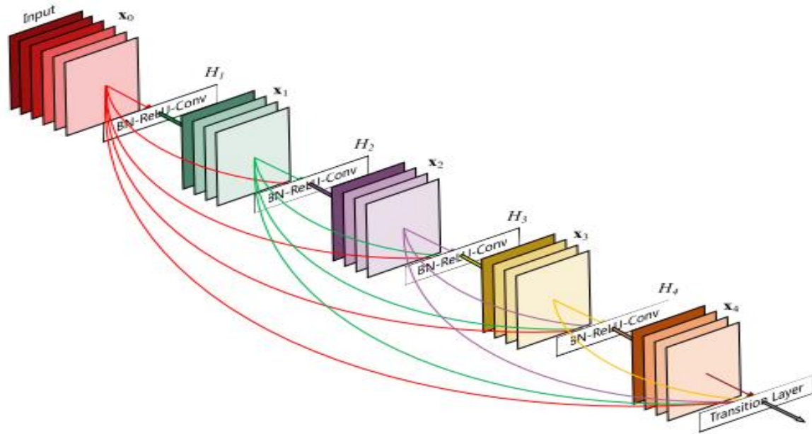
Figure 1. DenseNet Architecture(Huang., 2017)
