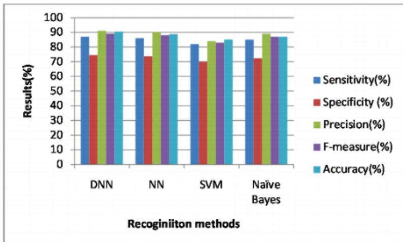
Figure 3.5. Proposed Algorithm Performance (Urdu)
