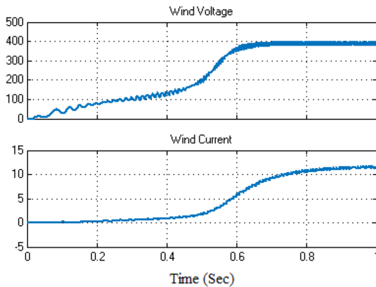
Fig. 9 Wind Voltage And Current
