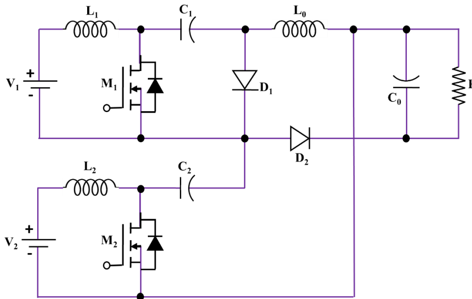
Fig. 2 Fused Cuk-Sepic Converter
