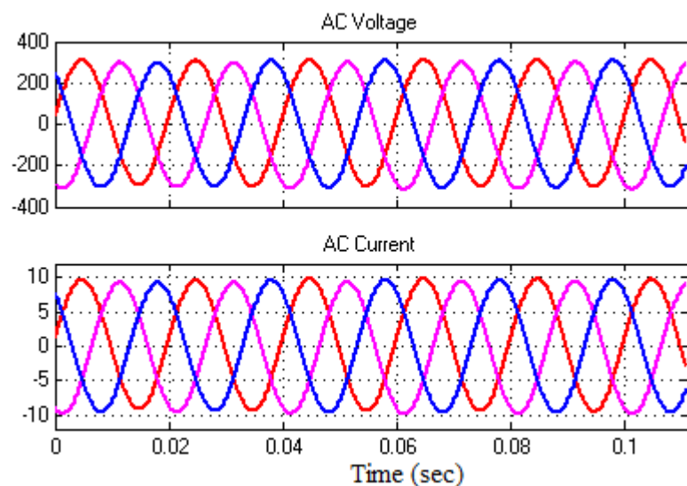
Fig. 11 Inverter Output
