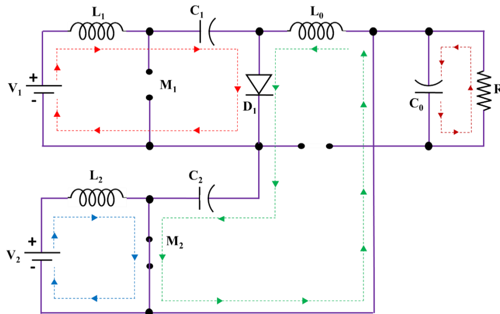
Fig. 5 Mode Iii Equivalent Circuit
