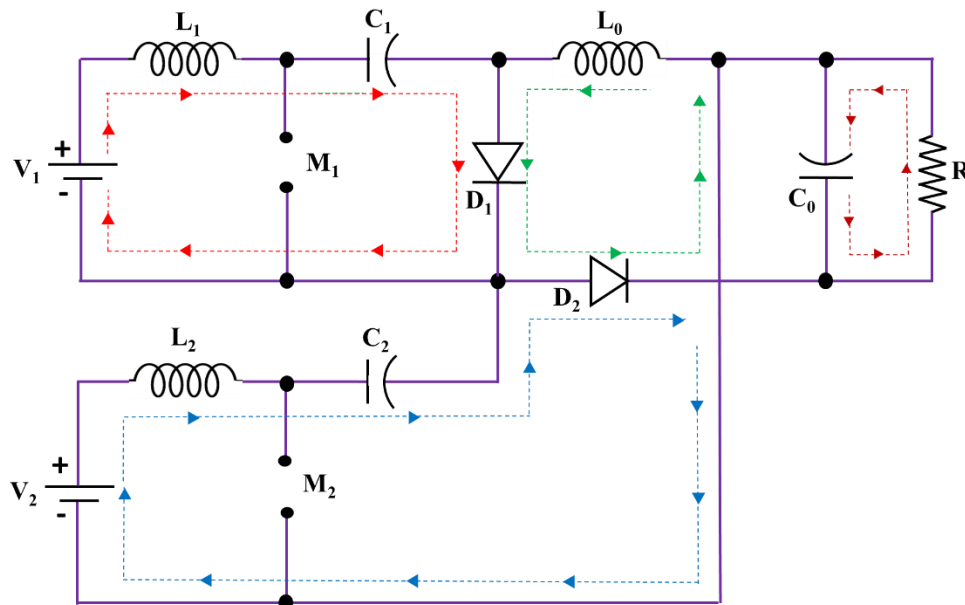
Fig. 6 Mode Iv Equivalent Circuit
