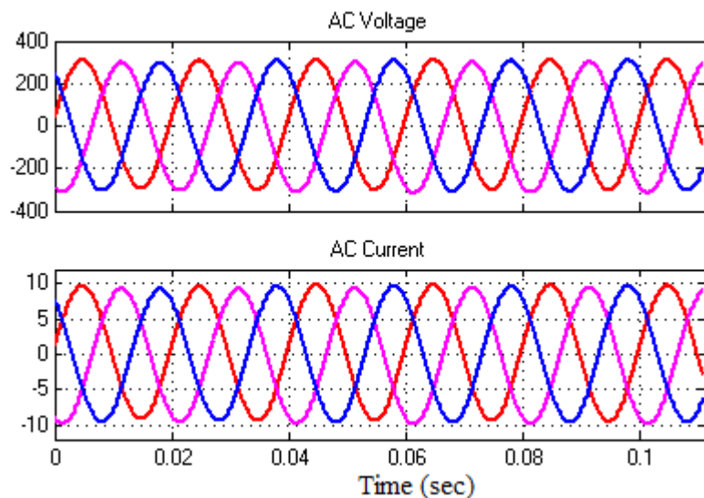
Fig. 11 Inverter Output
