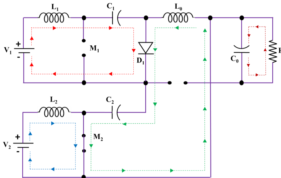
Fig. 5 Mode Iii Equivalent Circuit
