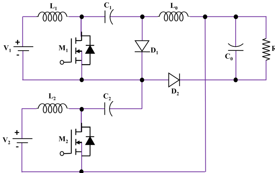
Fig. 2 Fused Cuk-Sepic Converter
