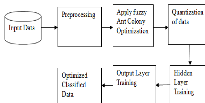
Fig 1. Overview of NBNFA
