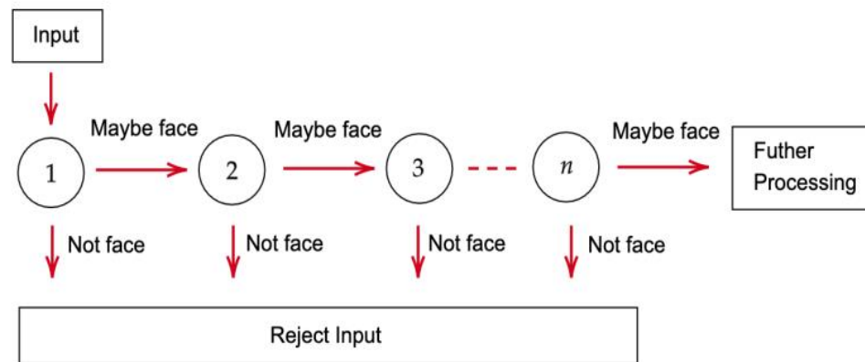
Figure 3: Algorithm Execution
