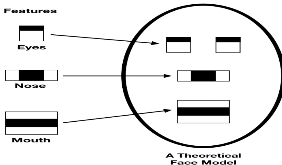
Figure 4: Feature Extraction
