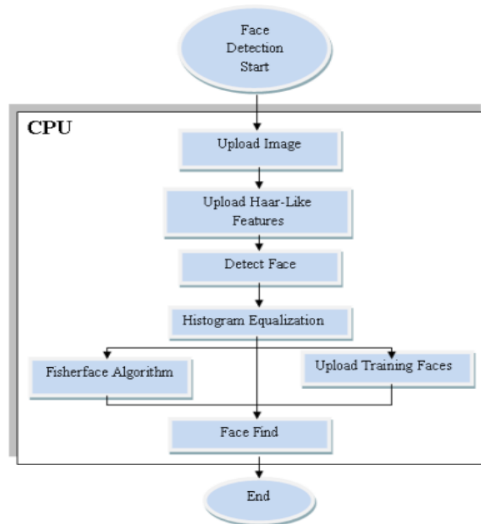
Figure 2: Block Diagram of Proposed Methodology
