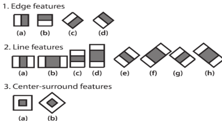
Figure 1: Haar Features
