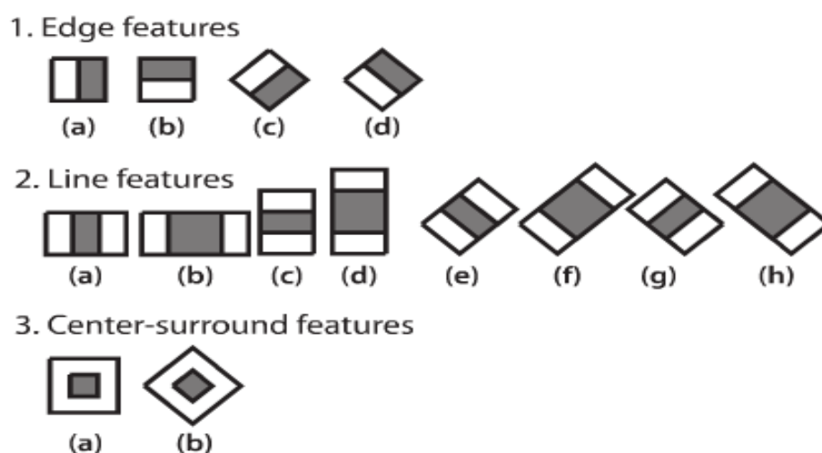
Figure 1: Haar Features
