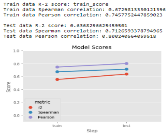
Figure.14.Training and Testing By Lasso Algorithm
