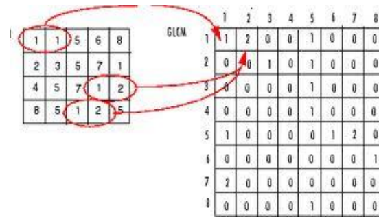
Figure 7: GLCM
