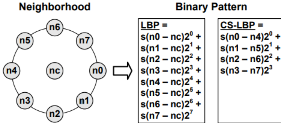
Figure 4: Description of CS-LBP
