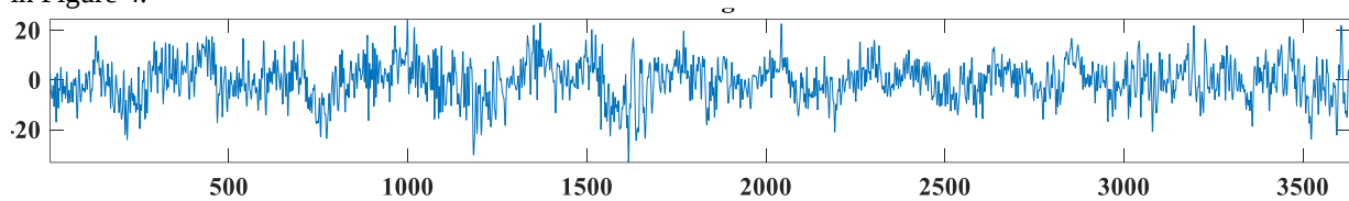
Figure 2: Normal EEG signal
