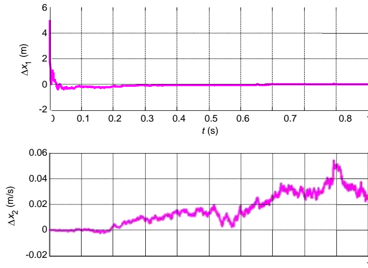
Figure 4. Kalman Filtering Example Estimation Errors
